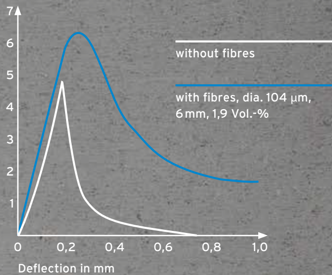
Peripheral stress in N/mm 2
